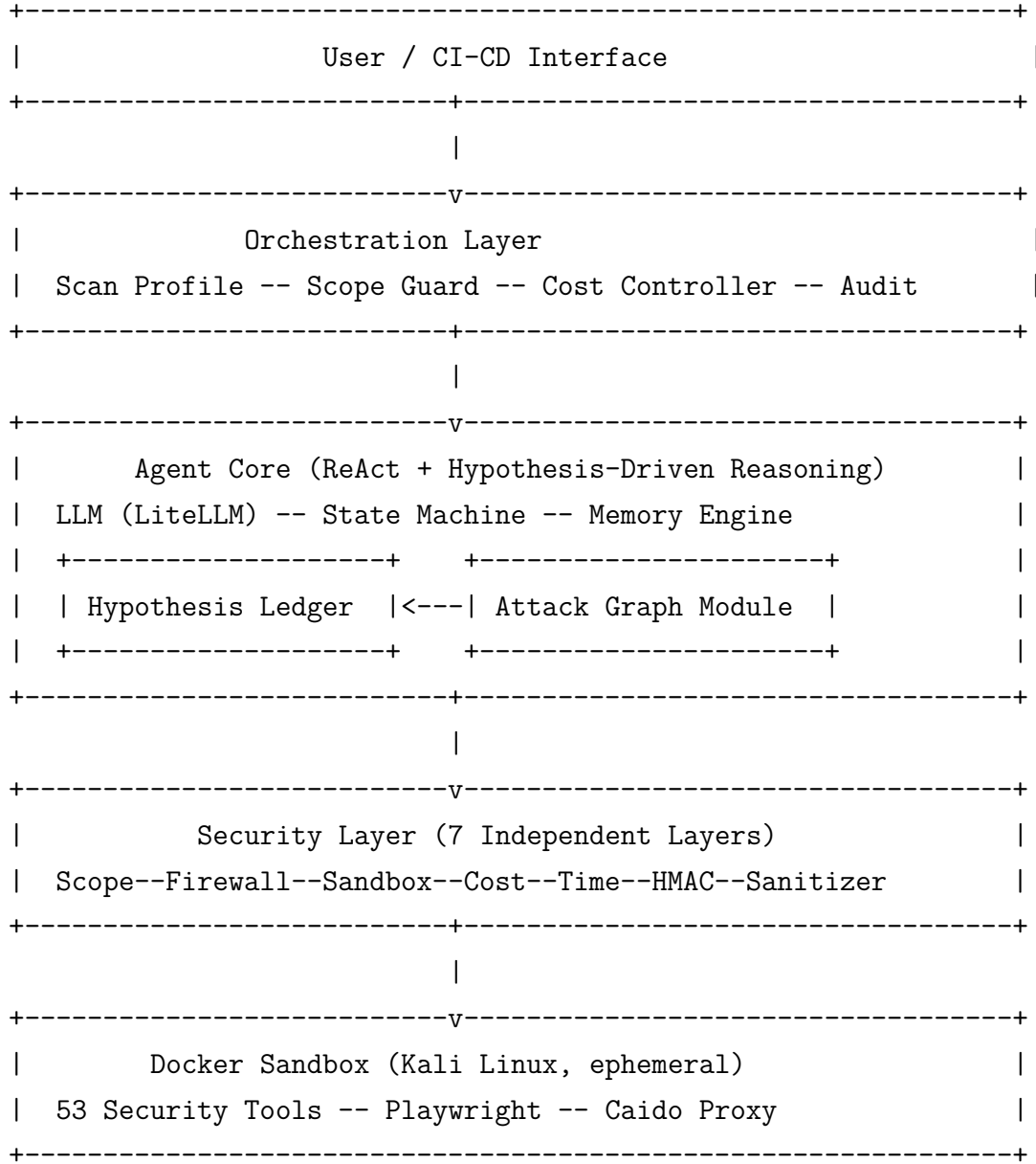
Figure 5.1: PHANTOM Conceptual Architecture (addressing Gaps G1–G6).
