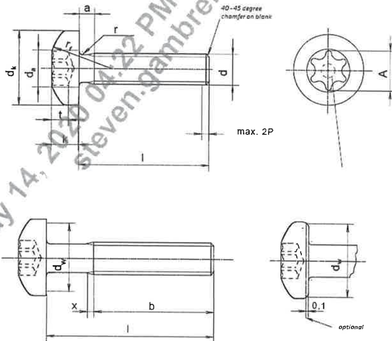
Figure 1 - Pan Head screws
