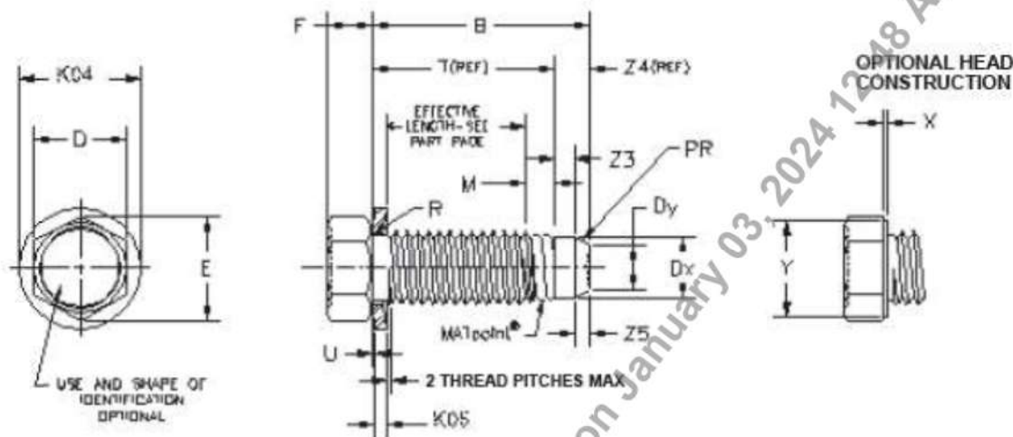
Figure 1 - Hexagon Head Screw & coned washer – Matpoint
