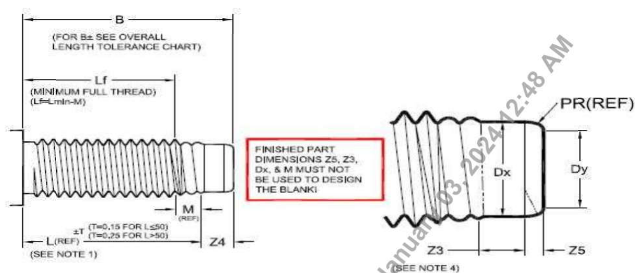
Figure 2 - Matpoint dimensional requirements
