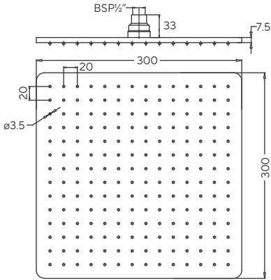
Q503146220 Overhead Shower 300x300mm in Chrome MRP: ₹ 14,990
