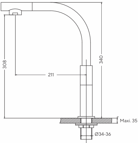
Q363118220 Zelos Single Function Pulldown Kitchen Faucet MRP: ₹ 16,990
