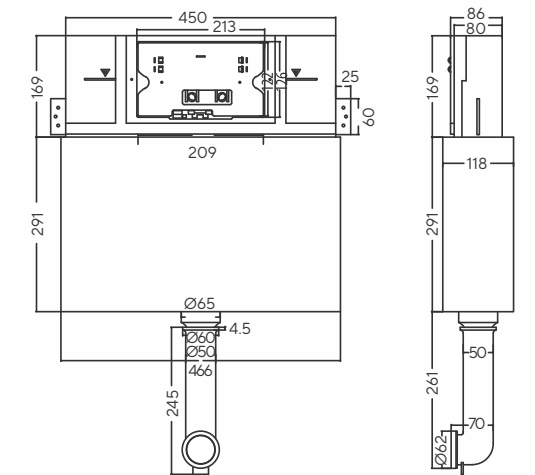
Q507451110 Concealed Cistern Sisma with Full Frame - QF MRP: ₹ 11,990
