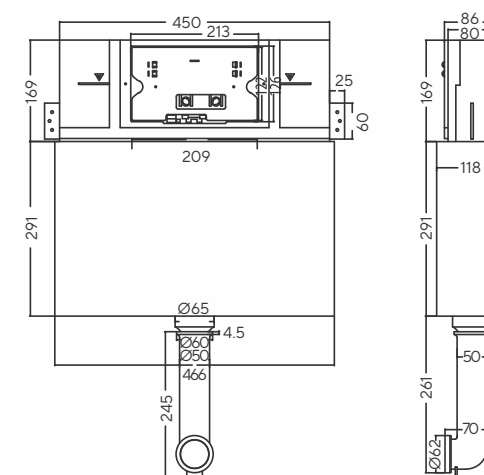
Q507451210 Concealed Cistern Sisma with Half Frame - QF MRP: ₹ 9,990
