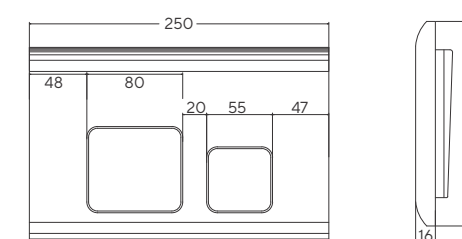
Q507455120 Sisma Flush Plate MRP: ₹ 1,790
