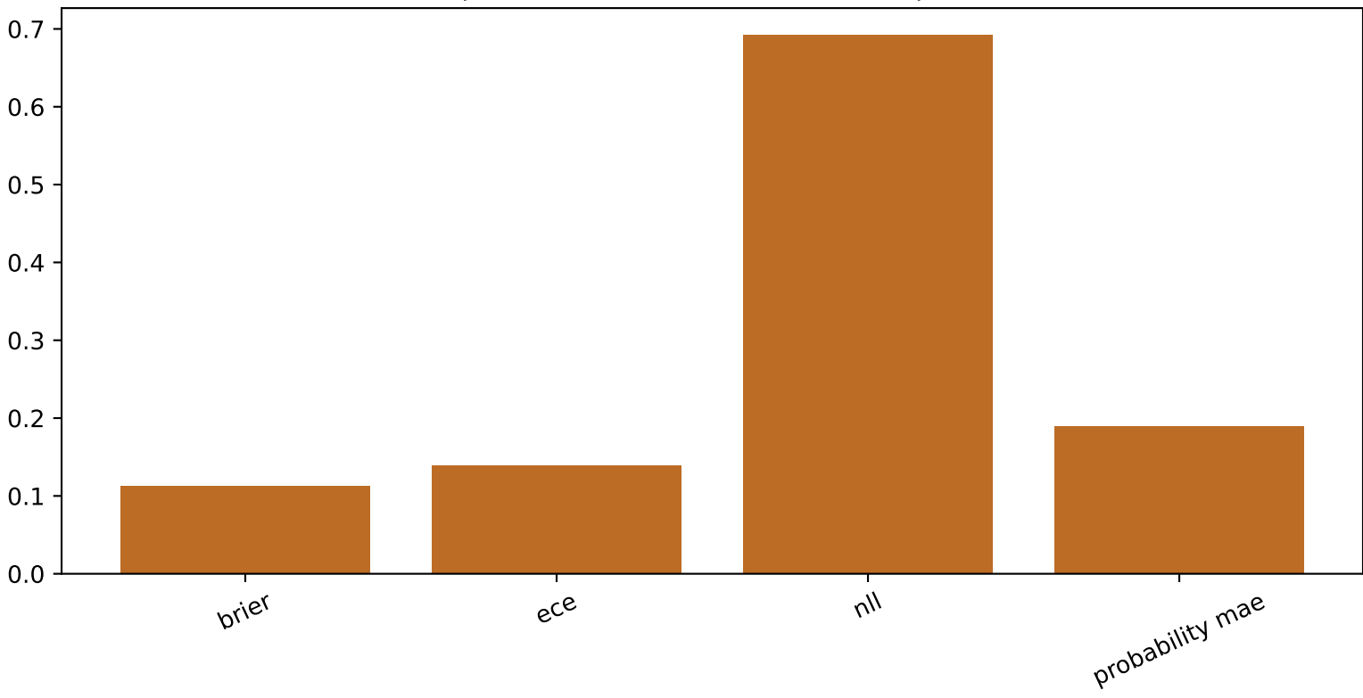
External probability quality B66 | frozen external ClinVar cohort | n=200
