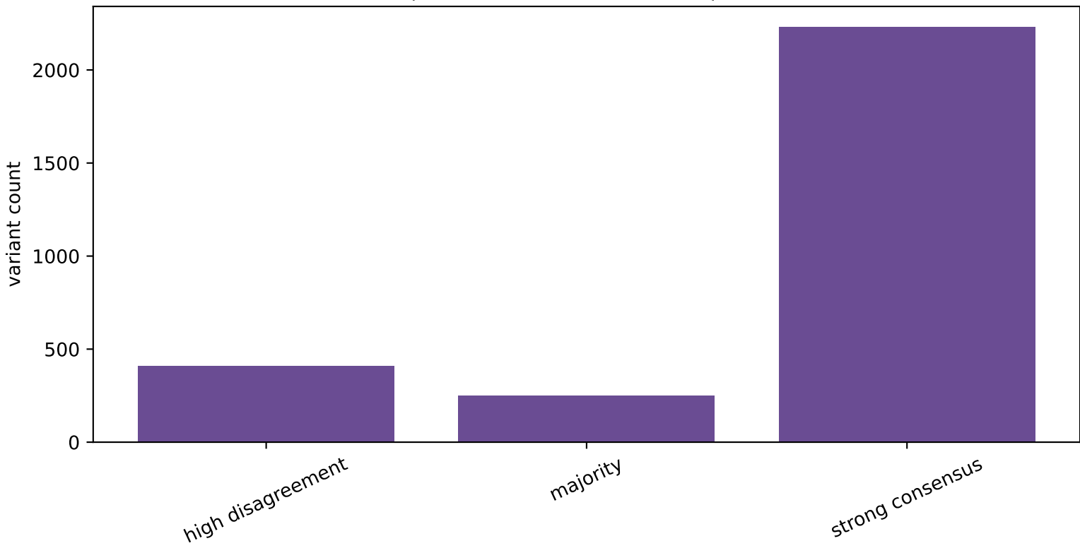
Model disagreement categories B49 | common validation rows | n=2891
