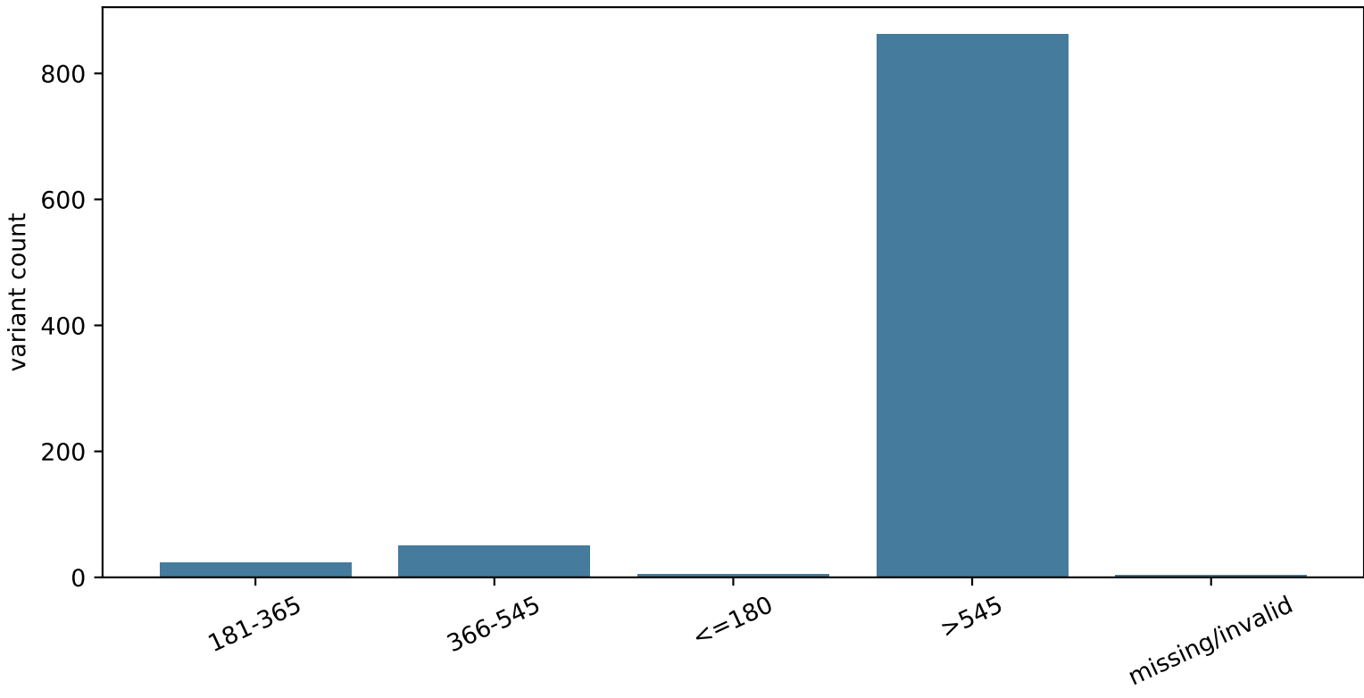
Temporal difficulty by resolution interval B47 | locked temporal cohort | n=946
