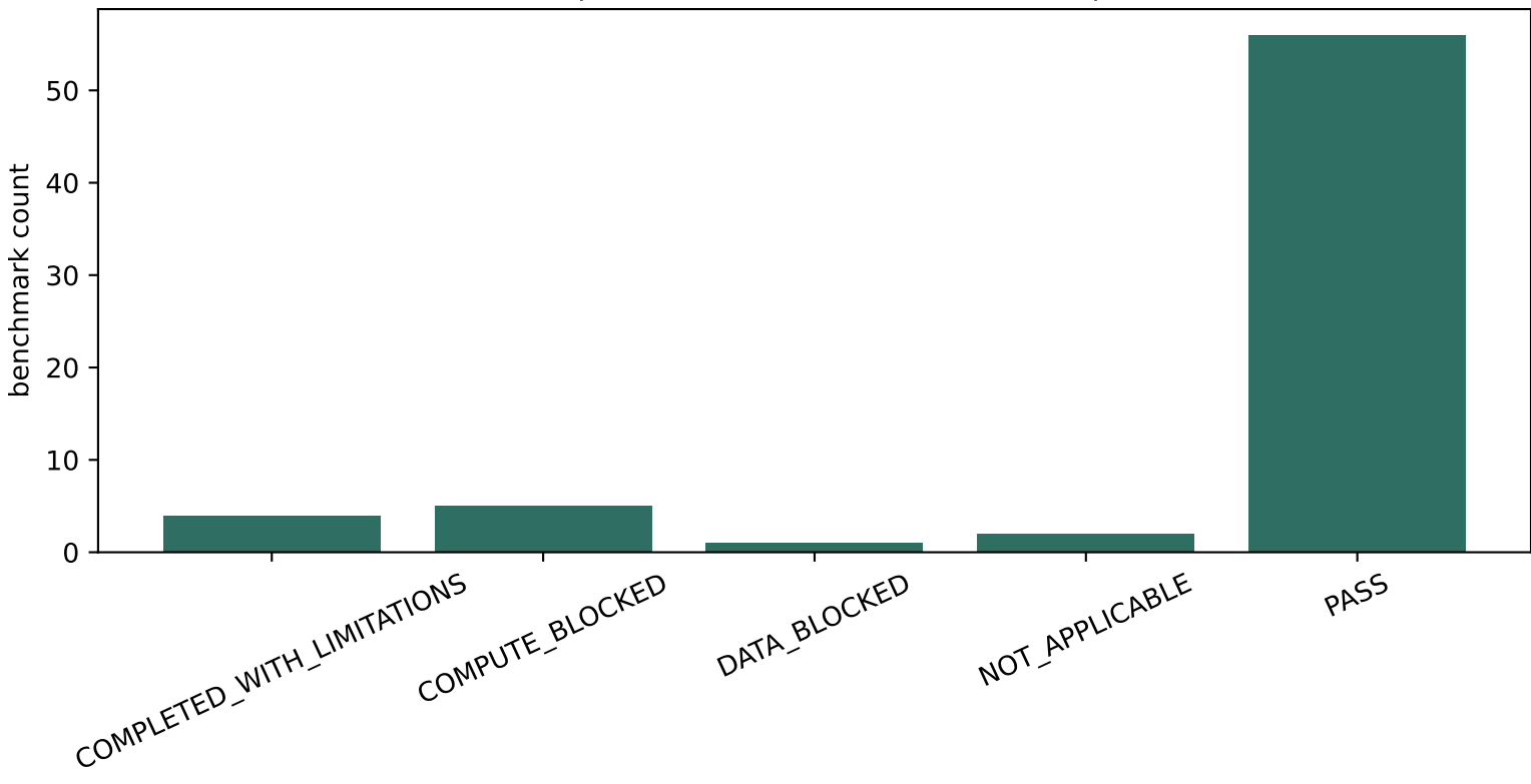
Benchmark status matrix B01-B68 | registered benchmark catalog | n=68
