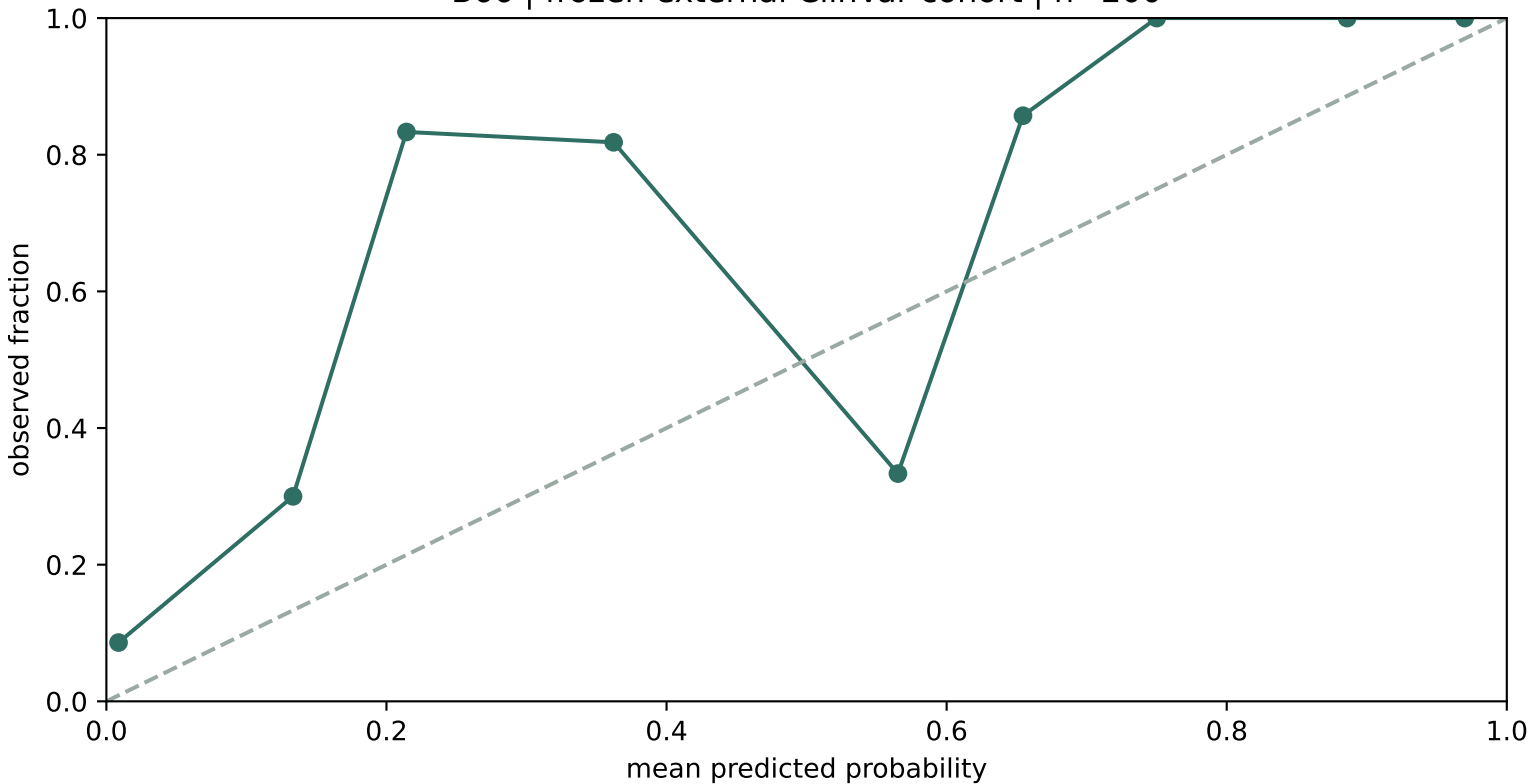
External calibration reliability B66 | frozen external ClinVar cohort | n=200
