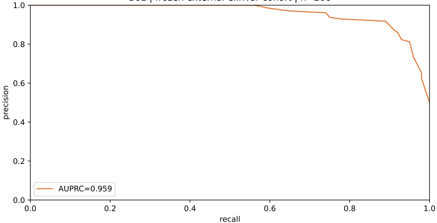
External precision-recall B61 | frozen external ClinVar cohort | n=200
