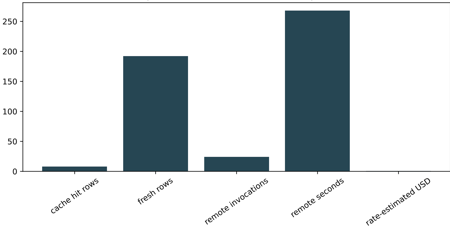
External runtime and cache economics B67 | frozen external ClinVar inference | n=200
