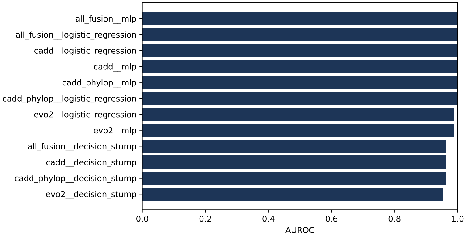
Validation model comparison B14 | formal validation split | n=595
