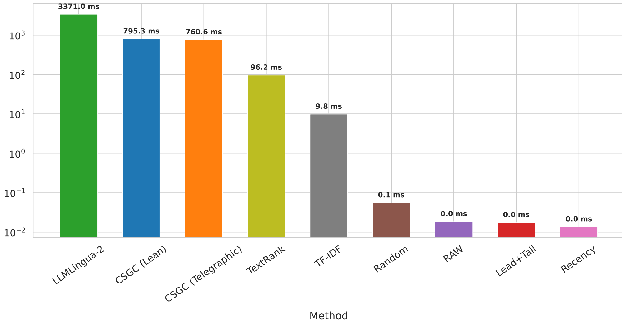
Figure 3 — Runtime per Method [30% budget, N=99]
