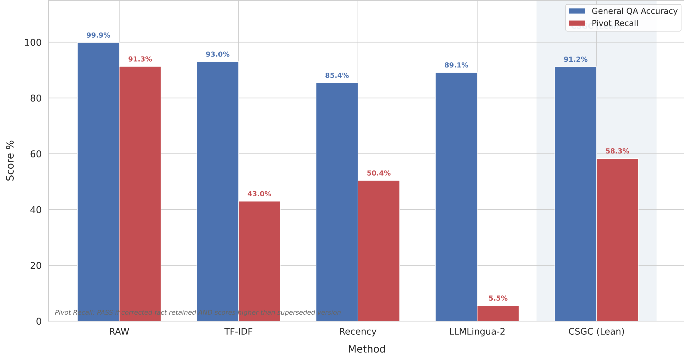
Figure 6 — General QA Accuracy vs. Pivot Recall @ 30% Budget (Pivot Recall: does compressed output preserve the CORRECTED fact over the superseded one?)
