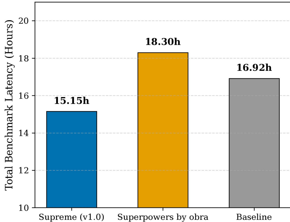
B: Total Wall-Clock Latency (Lower is Better)
