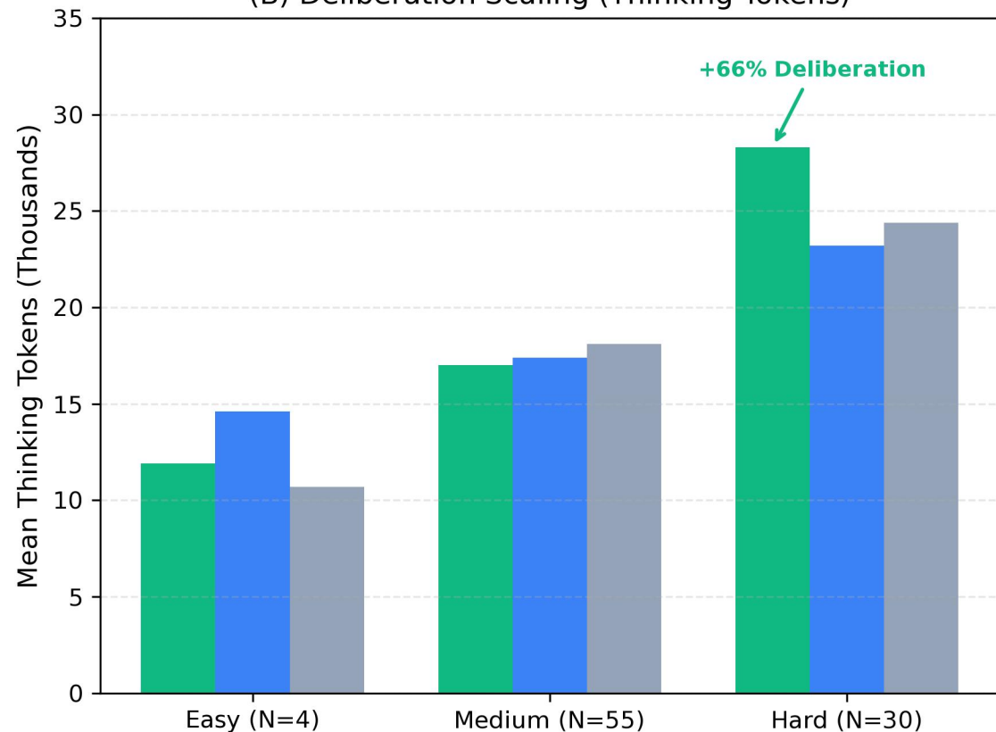
(B) Deliberation Scaling (Thinking Tokens)
