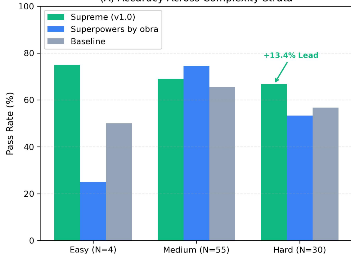
(A) Accuracy Across Complexity Strata
