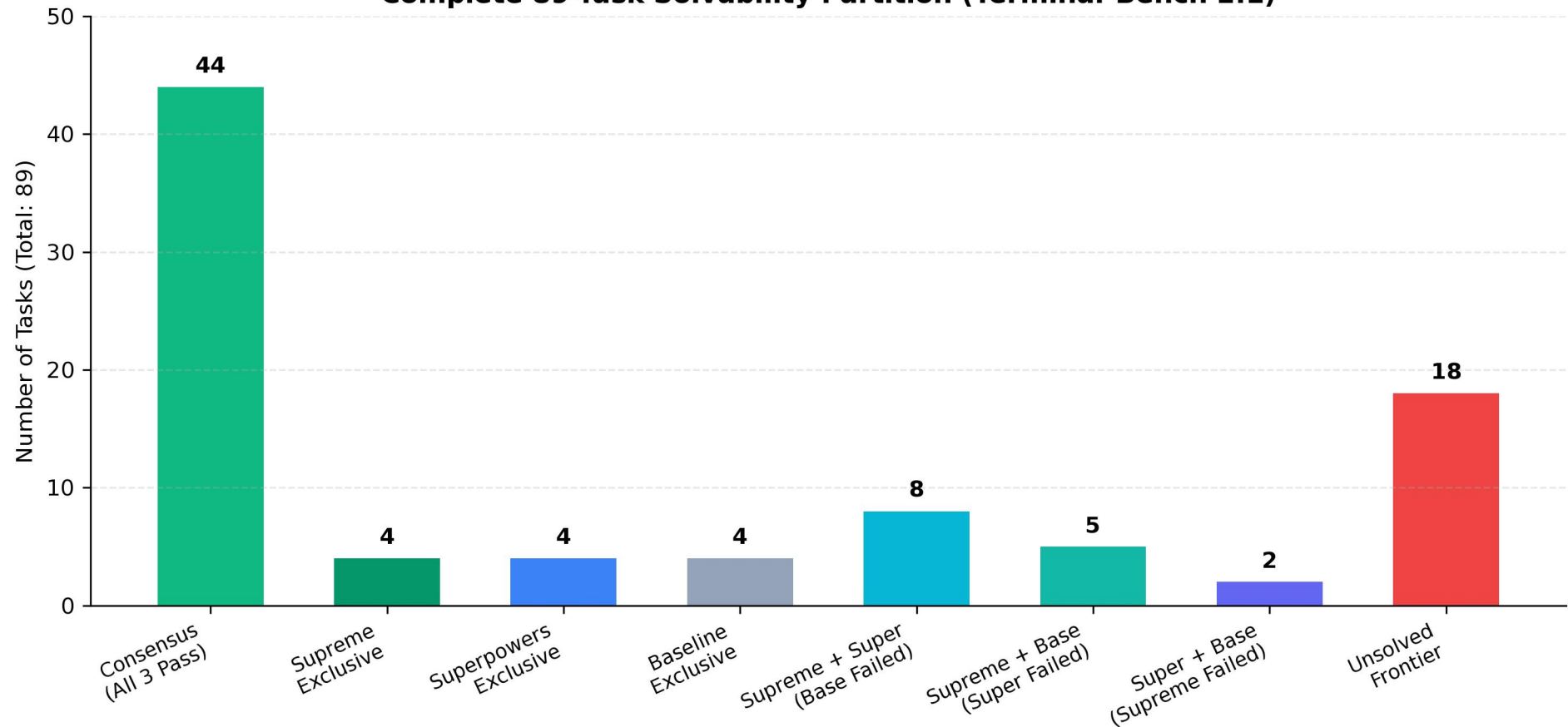
Complete 89-Task Solvability Partition (Terminal-Bench 2.1)
