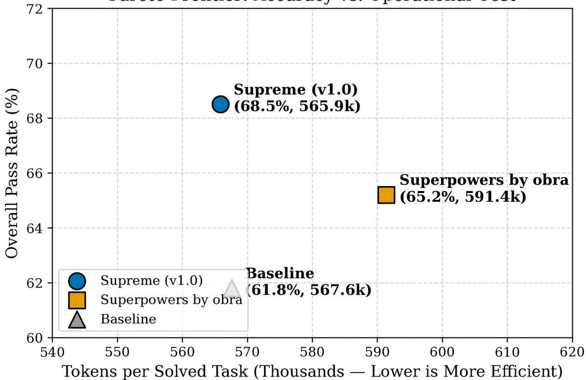
Pareto Frontier: Accuracy vs. Operational Cost
