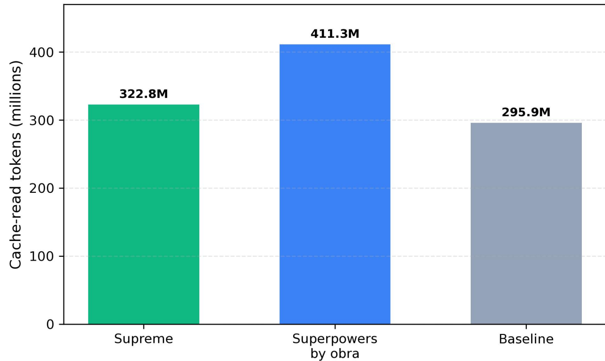
(B) Provider-reported cache reads
