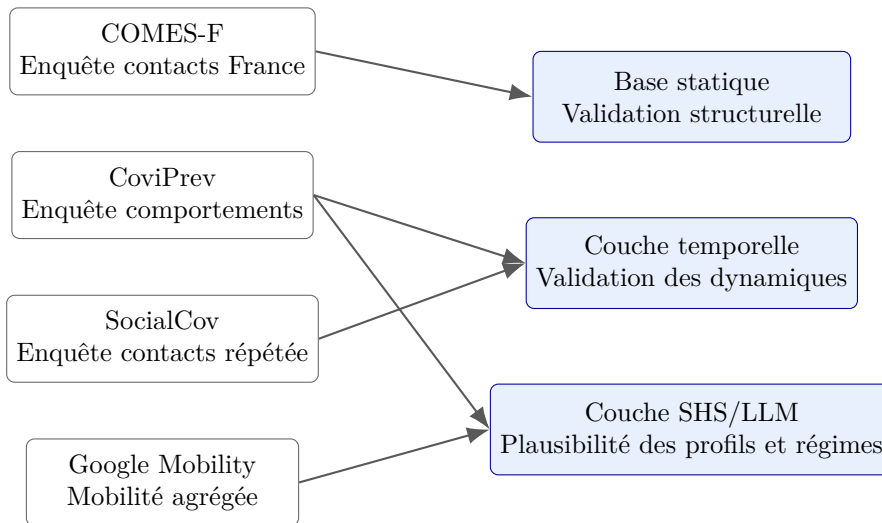
FIGURE 2 – Comment les sources empiriques alimentent le pipeline.
