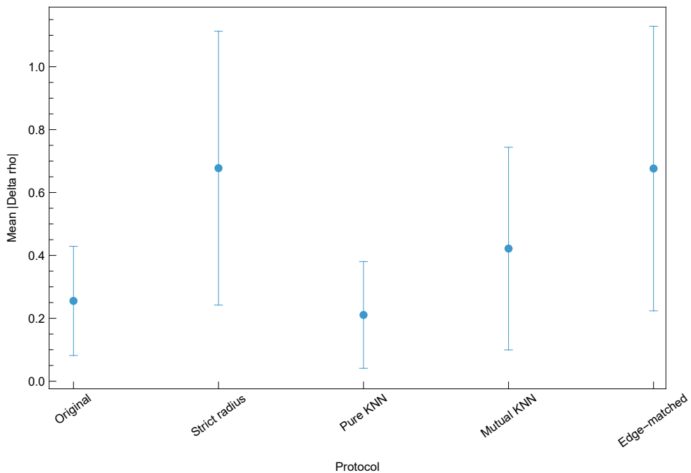
Bardeen five-protocol anchor (mean \pm SD)
