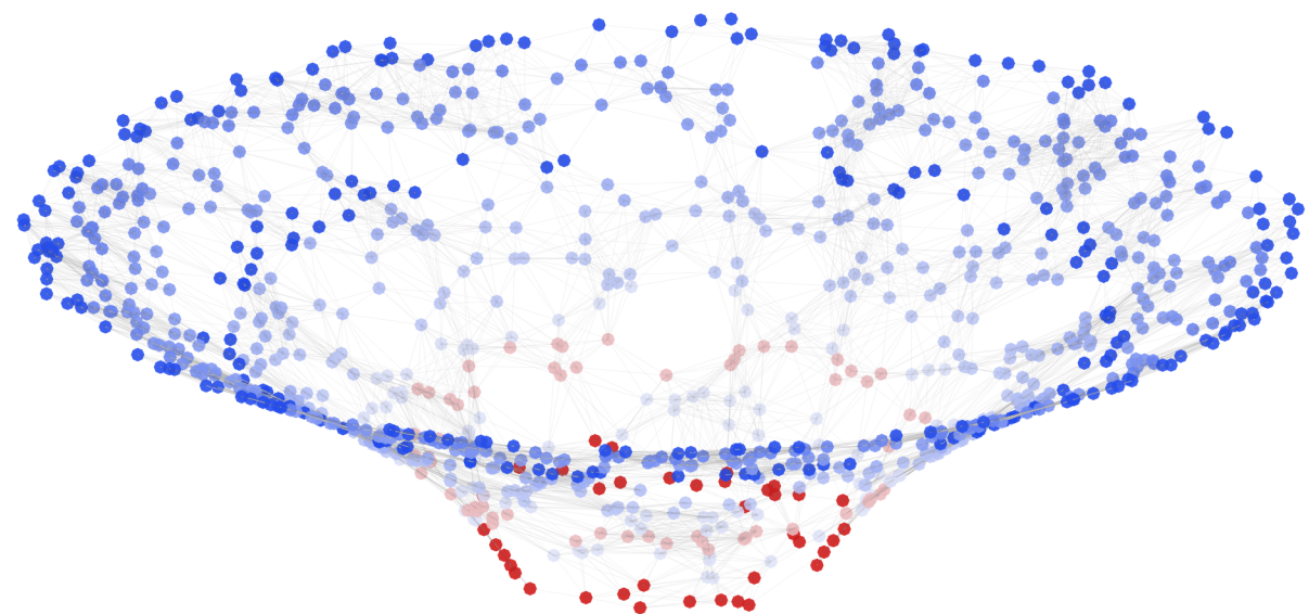
Hayward, scl = 0.2
