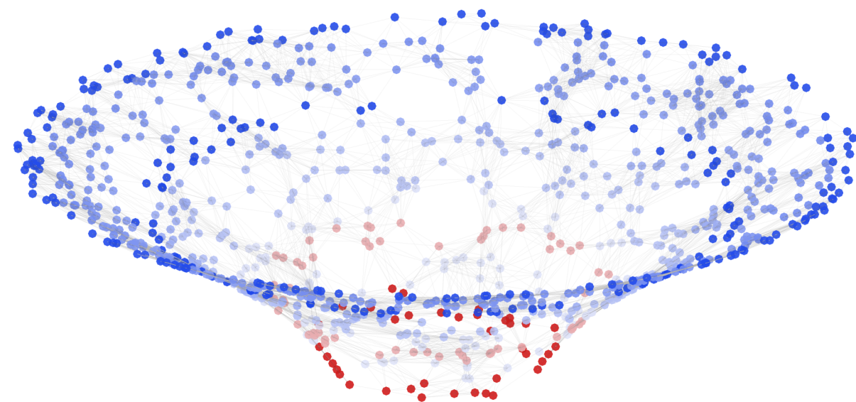
Bardeen, g = 0.2
