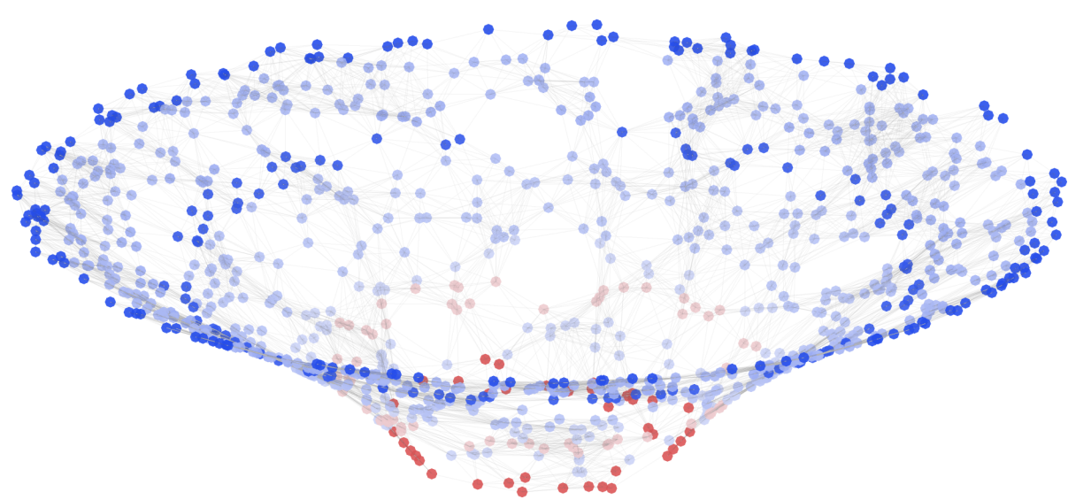
Reissner–Nordström, Q = 0.4
