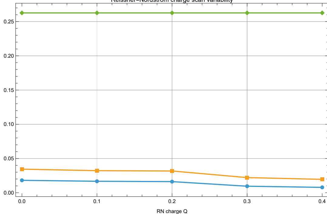
Reissner–Nordström charge scan variability
