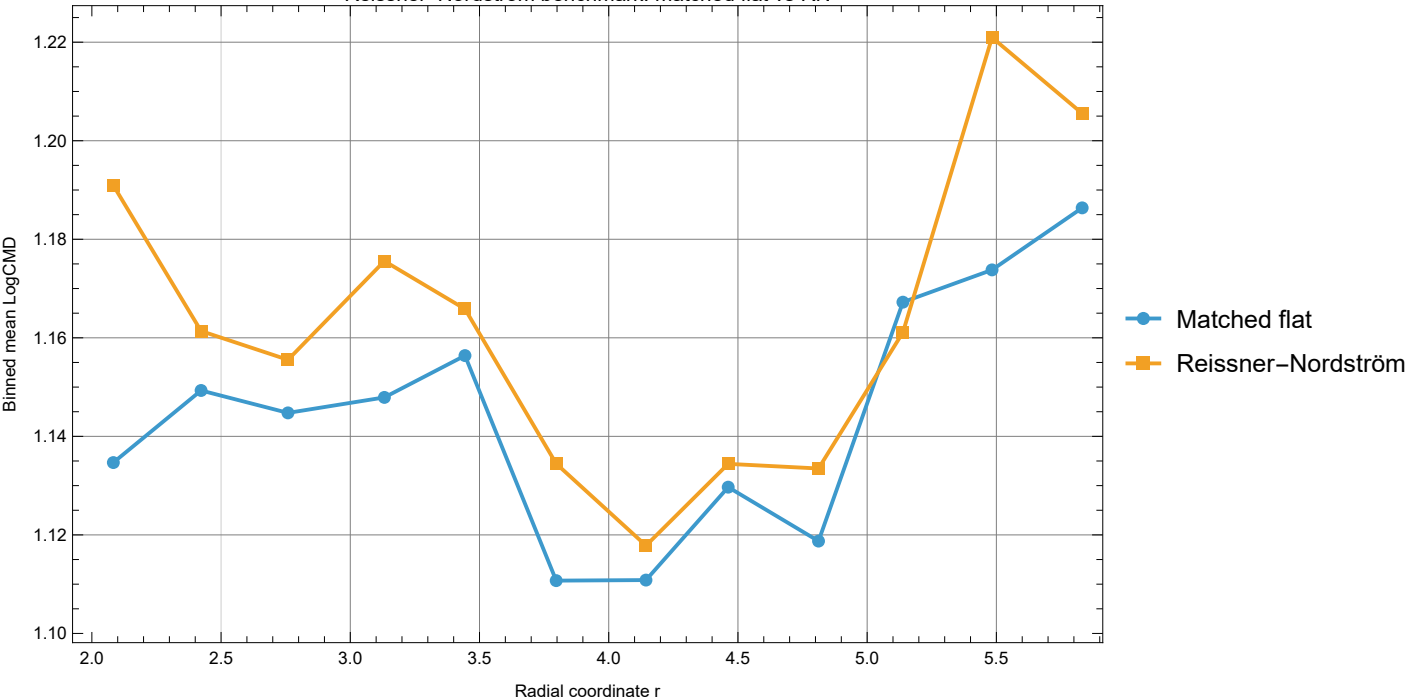
Reissner–Nordström benchmark: matched flat vs RN
