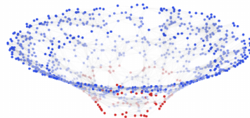
Hayward, l = 0.2
