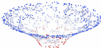
Bardeen, g = 0.2
