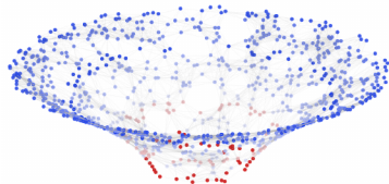
Schwarzschild/Flamm
