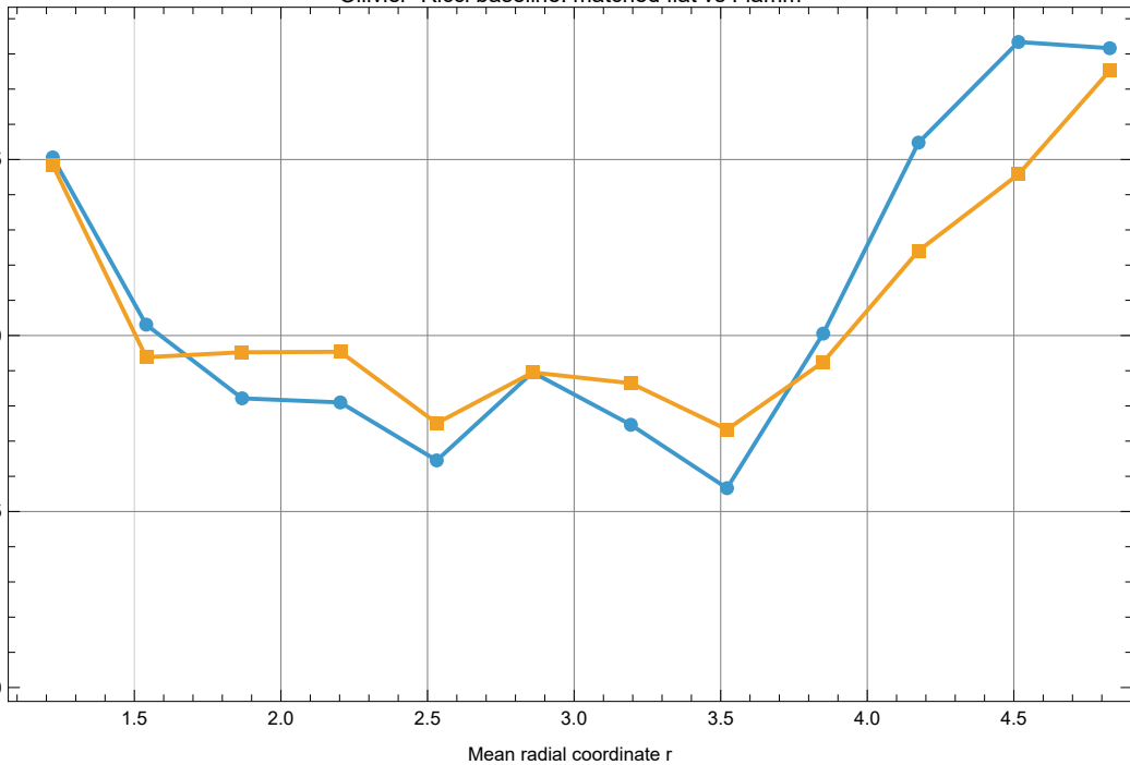
Ollivier–Ricci baseline: matched flat vs Flamm
