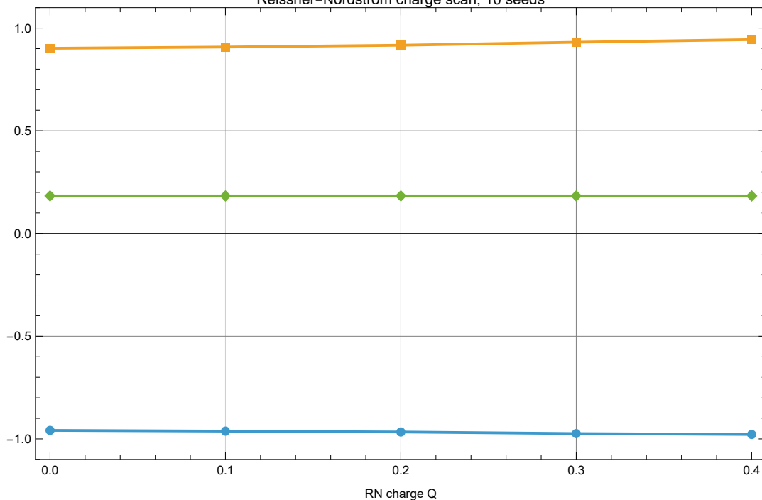
Reissner-Nordström charge scan, 10 seeds
