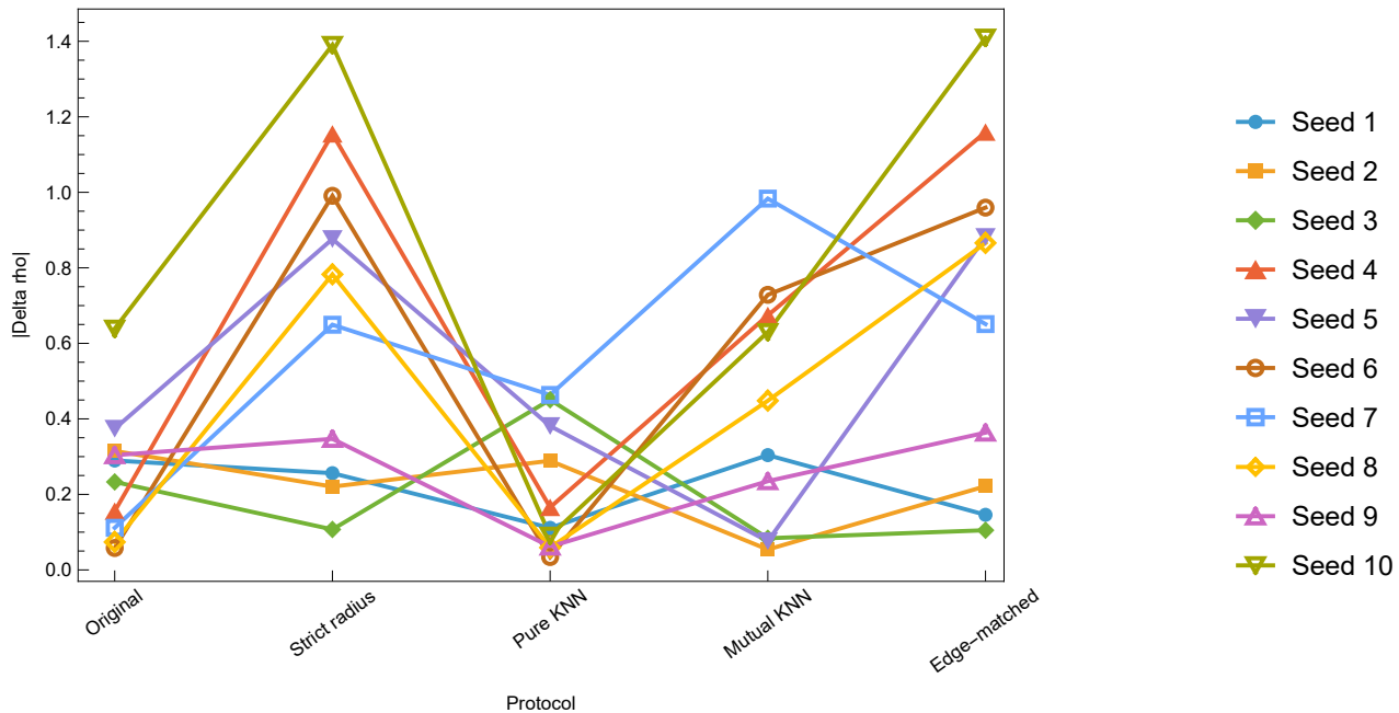
Bardeen paired absolute gaps
