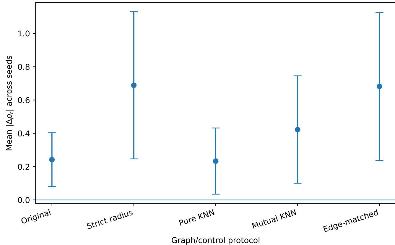
Construction sensitivity of shortest-path anisotropy
