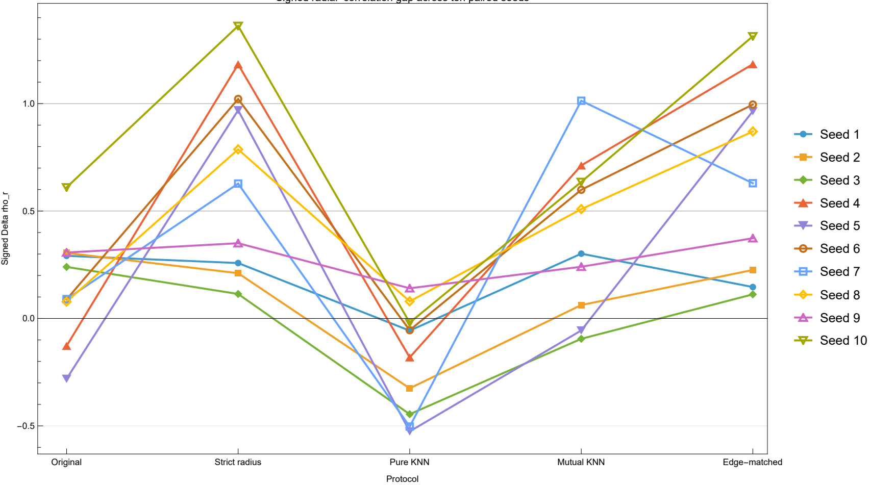
Signed radial-correlation gap across ten paired seeds
