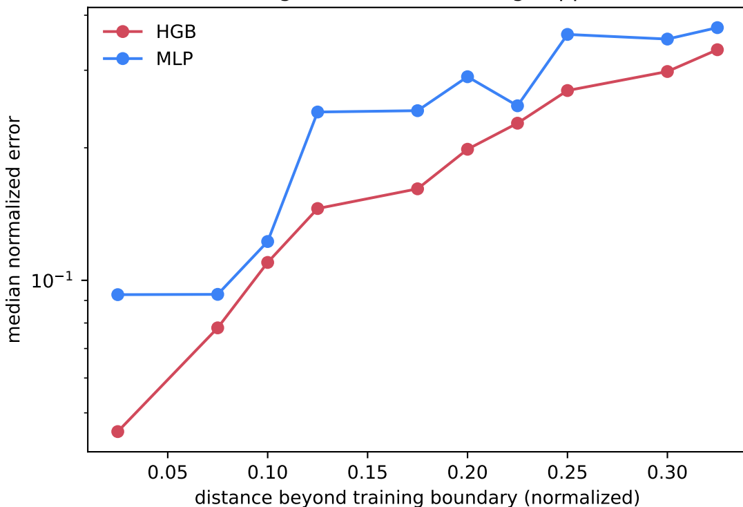
Error grows outside training support
