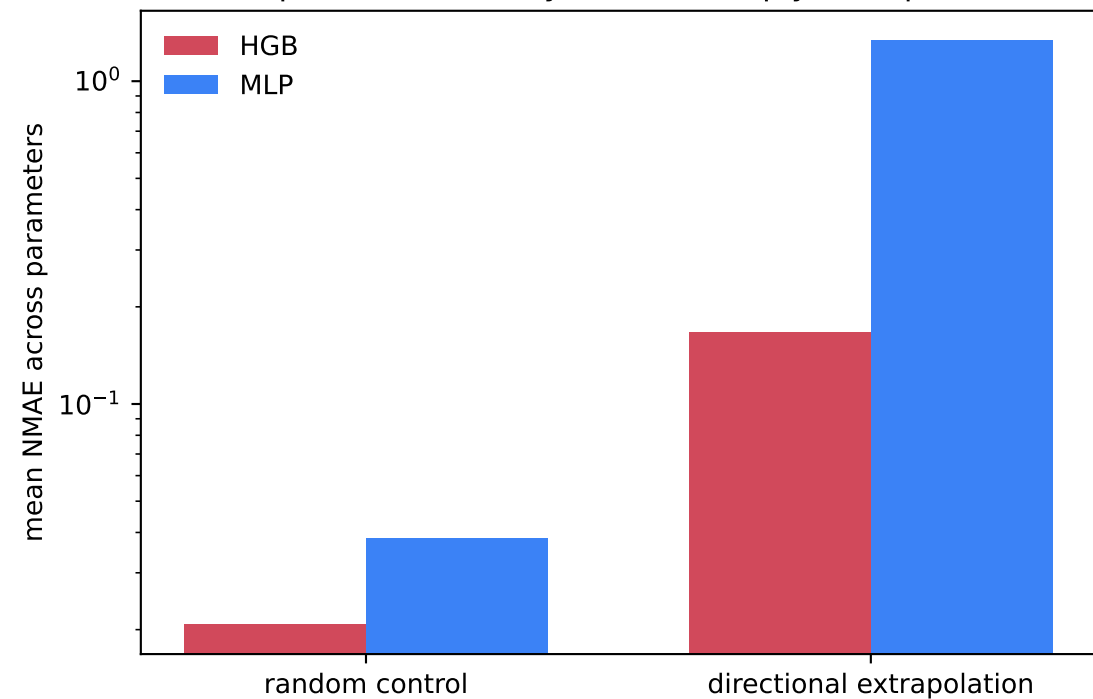
Interpolation accuracy does not imply extrapolation
