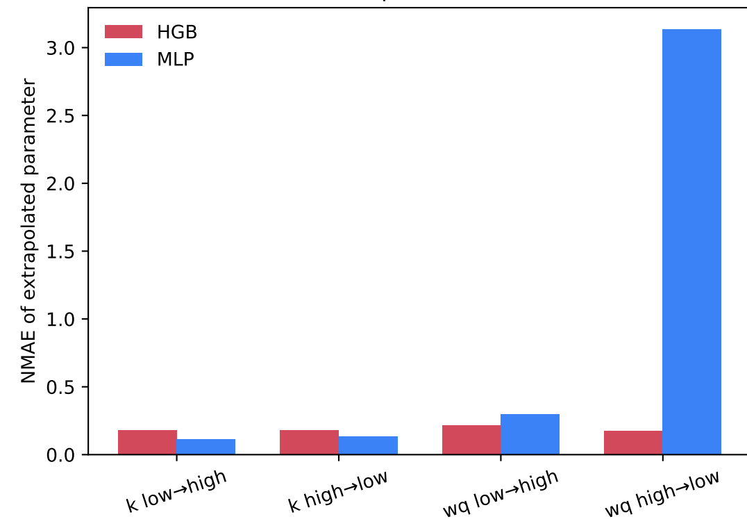
Error grows outside training support
