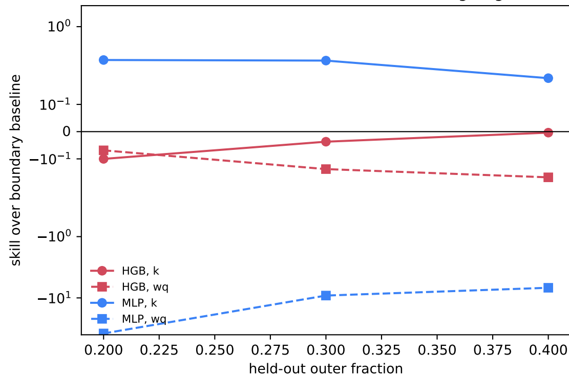
Interpolation accuracy does not imply extrapolation
