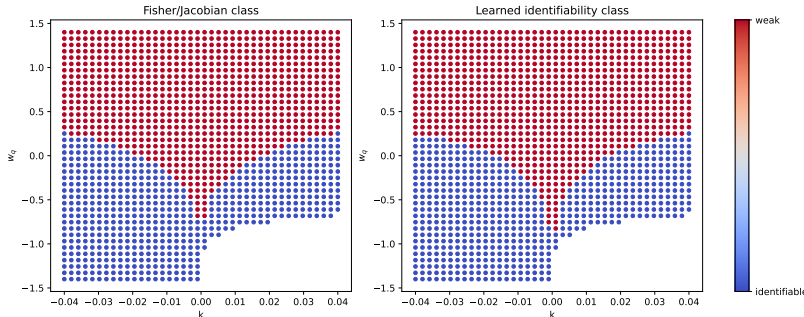
Figure 11: Historical dense synthetic rank-aware identifiability boundary. Exact k = 0 rank loss is structural, whereas the finite-width weak-identifiability region depends on precision. This historical benchmark motivated, but does not replace, the validated physical shooting analysis.
