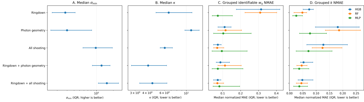
Figure 9: Aligned physical and empirical diagnostics: median minimum singular value, median condition number, grouped identifiable- w_q NMAE, and grouped k NMAE. Exact statistics and the feature order are shared across panels.
