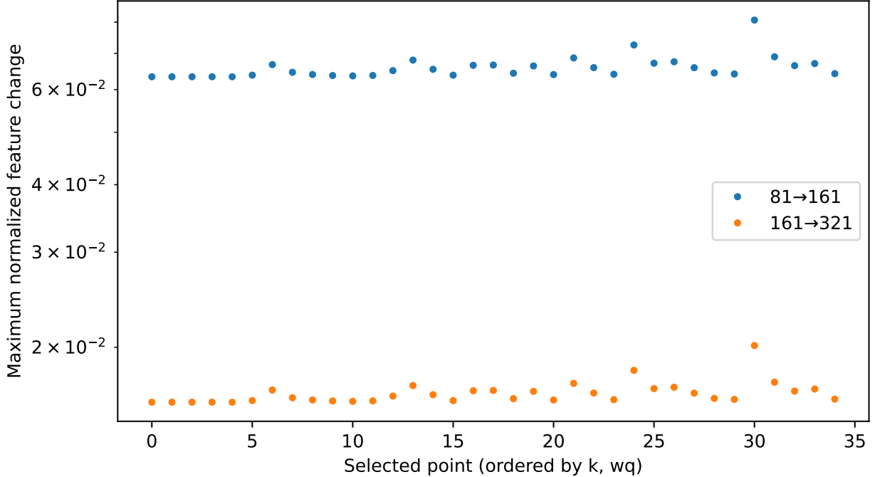
Figure 10: Targeted pointwise maximum normalized feature changes from 81 to 161 and 161 to 321 phases. The 321-phase audit resolves the forward-feature criterion but does not by itself certify inverse estimators.
