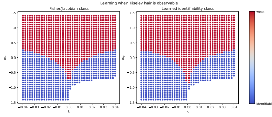
Figure 1: Rank-aware identifiability boundary in the historical dense synthetic domain. Exact k = 0 rank loss is separated from finite-precision weak identifiability.
