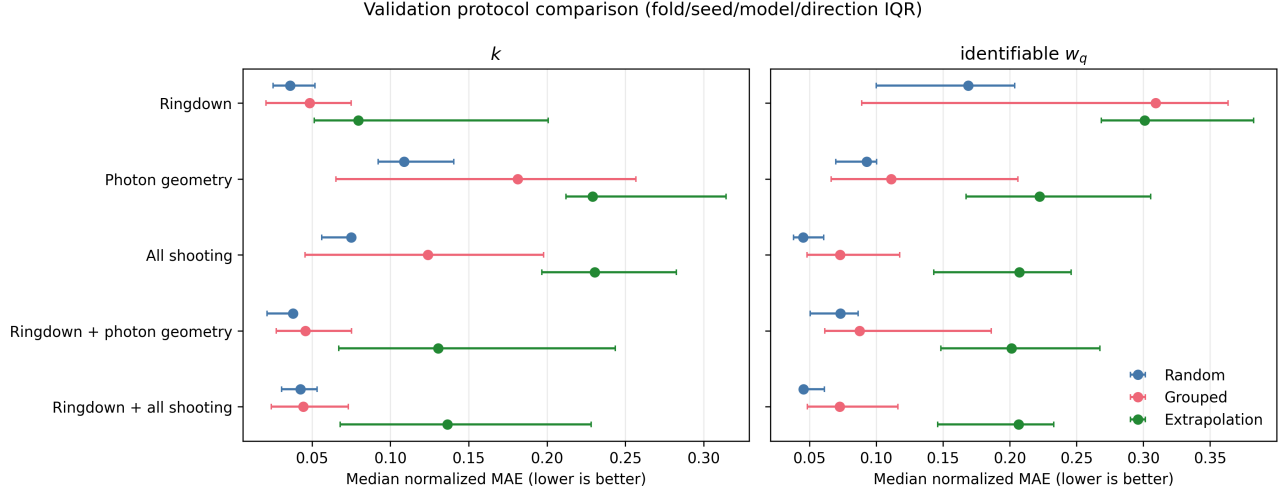
Figure 7: Median NMAE for the five primary feature sets under random, grouped physical interpolation, and directional extrapolation. Directions remain separate in the machine-readable source before aggregation.
