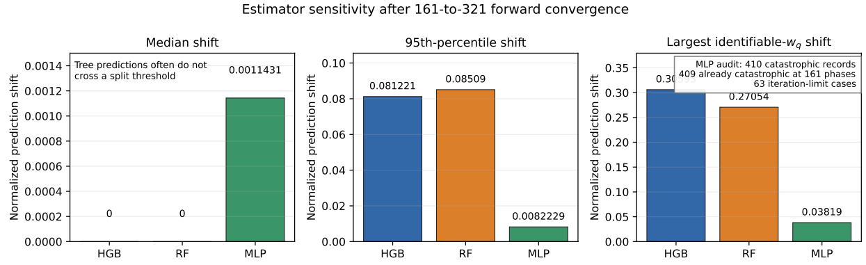
Figure 11: Frozen-estimator sensitivity after forward convergence. Bars show the median, 95th-percentile, and largest identifiable- w_q normalized prediction shift for HGB, RF, and MLP. The annotation records the distinct MLP failure audit: 410 catastrophic directional records, 409 already catastrophic at 161 phases, and 63 iteration-limit cases. No predictions are clipped.
