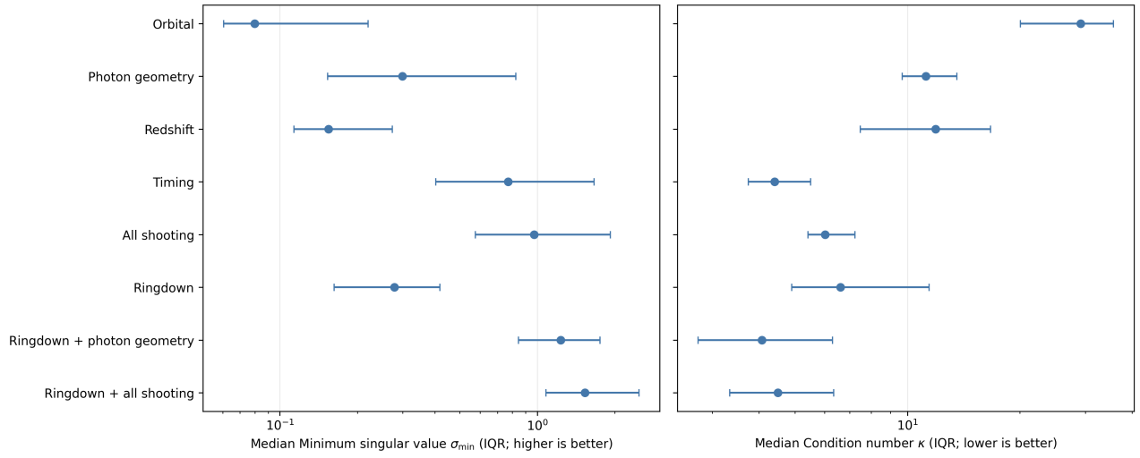
Figure 6: Grid-wide median and interquartile summaries of \sigma_{\min} and condition number. Photon geometry provides the clearest complement to ringdown.
