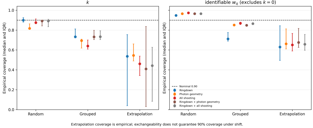
Figure 9: Empirical 90% split-conformal coverage by target and protocol. Ordinary w_q coverage excludes k = 0 ; extrapolation coverage is not guaranteed under distribution shift.
