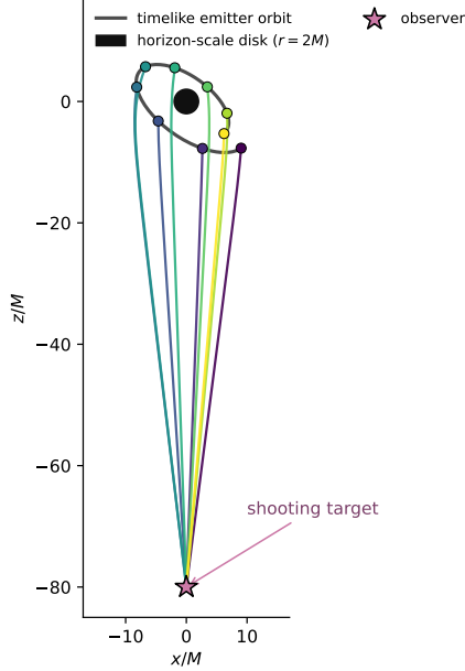
Direct Kiselev photon shooting from an orbiting emitter
