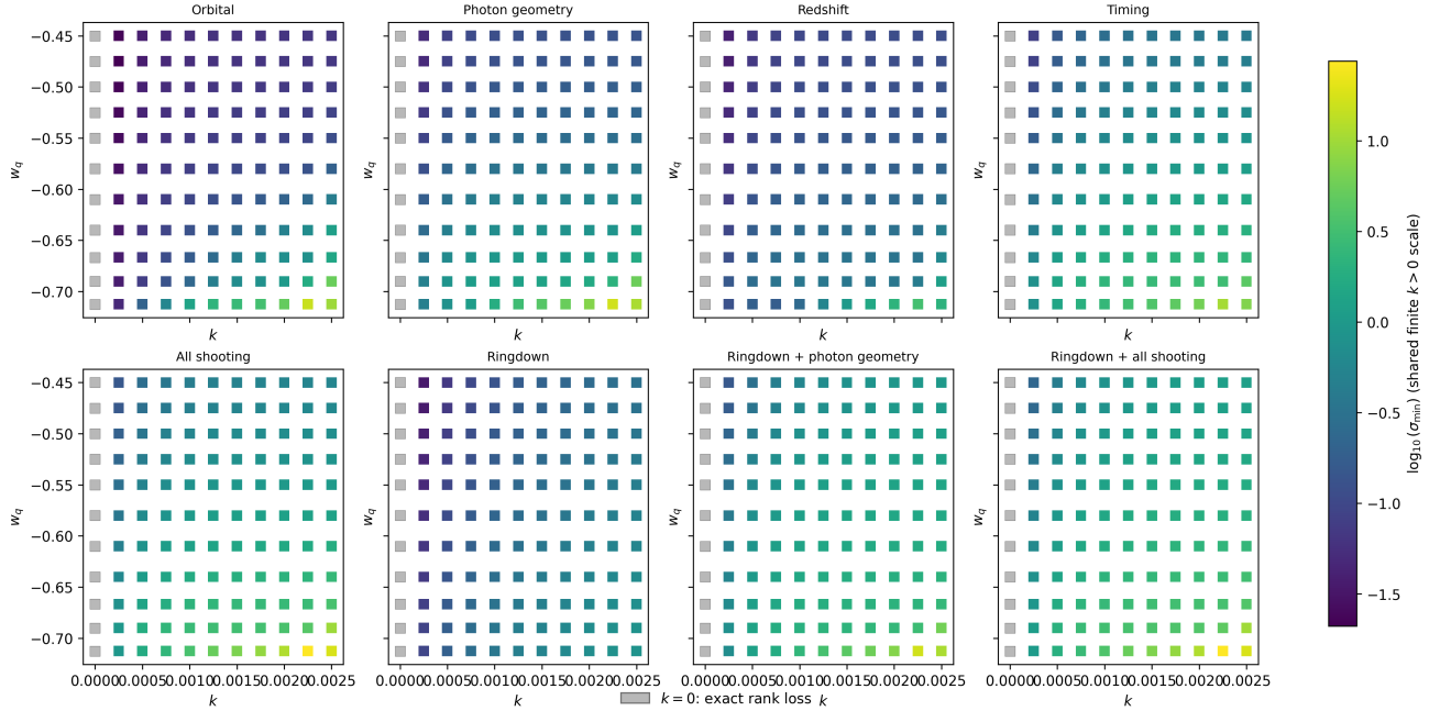
Figure 5: Grid maps of \log_{10} \sigma_{\min} with exact k = 0 rank-loss points masked. Missing or invalid values are not interpolated, and all panels use one finite- k color scale.
