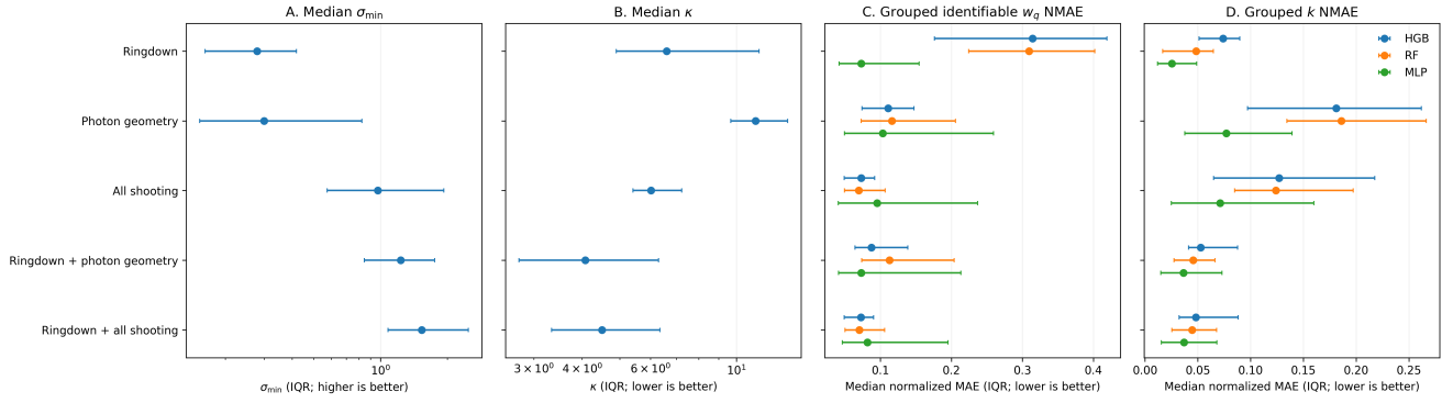
Figure 8: Aligned physical and empirical diagnostics: median minimum singular value, median condition number, grouped identifiable- w_q NMAE, and grouped k NMAE. Exact statistics and the feature order are shared across panels.
