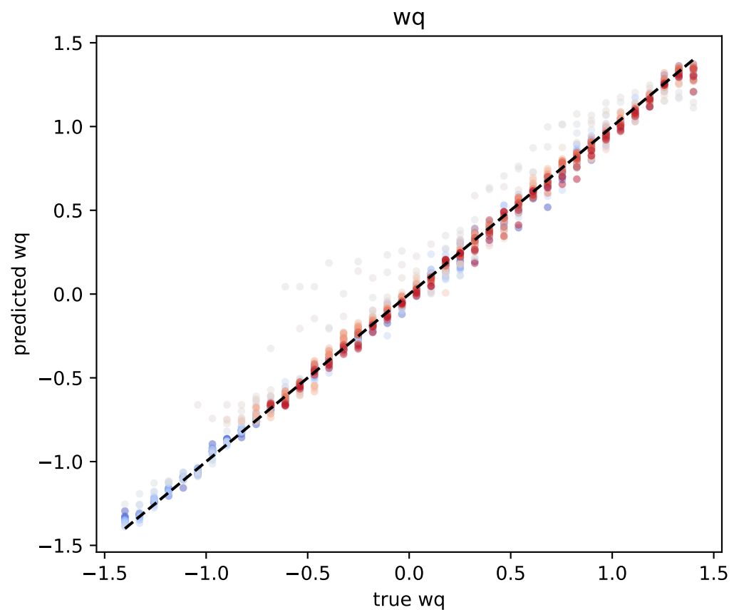
Waveform-to-hair grouped predictions (HistGradientBoostingRegressor)
