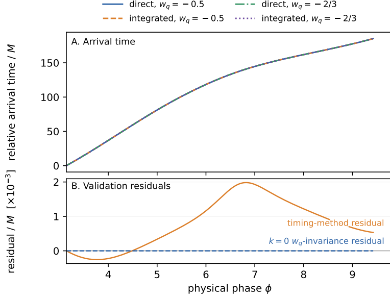
Figure 15: Schwarzschild arrival-time validation. The four phase-resolved series are the direct and redshift-integrated arrival-time constructions for each of two nominal w_q values. At k = 0 those values describe the same Schwarzschild geometry. In the lower panel, the orange residual checks timing consistency, T_{\text{direct}} - T_z , where T_z = \int (1 + z) d\tau_{\text{emit}} , and the blue residual checks exact k = 0 w_q invariance, T_{\text{direct}}(w_q = -0.5) - T_{\text{direct}}(w_q = -2/3) . Both are shown on their actual numerical scales. The independently integrated T_z is a validation quantity, not the timing feature used for ML inference.
