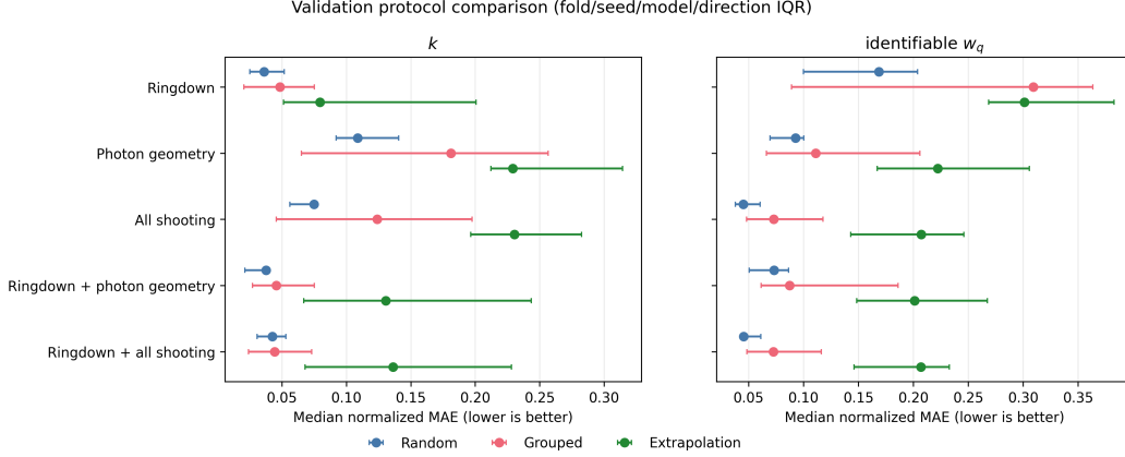
Figure 5: NMAE for the five primary feature sets under random, grouped physical interpolation, and directional extrapolation. Each dot preserves the predefined table statistic: the median of archived summary-row medians. To expose lower-level dispersion rather than suppress it through that hierarchy, each horizontal bar spans the 25th–75th percentile of the underlying NMAE records across the applicable folds, seeds, models, and, for extrapolation, directions. Thus the point and bar intentionally summarize different aggregation levels; directions remain separate in the machine-readable source before aggregation.
