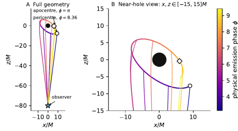
Figure 2: Representative direct-branch null geodesics for M = 1 , r_p = 8M , r_o = 12M , k = 10^{-3} , w_q = -0.5 , and observer (0, 0, -80M) . Physical phase runs from \pi at apocentre to 3\pi ; the diamond marks the numerically detected pericentre and the dark disk is a horizon-scale marker, not a shadow. At each phase, two launch angles are solved until the ray reaches the observer. The right panel shows the stated near-hole coordinate bounds on their actual scale; no trajectory is geometrically magnified. This is a controlled dimensionless benchmark.
