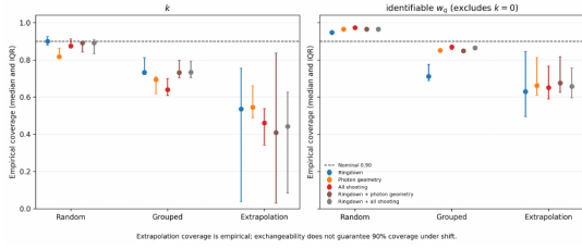
Figure 10: Empirical 90% split-conformal coverage by target and protocol. Ordinary w_0 coverage excludes k = 0 ; extrapolation coverage is not guaranteed under distribution shift.
