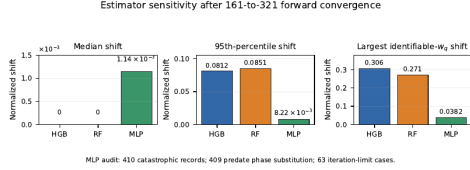
Figure 12: Frozen-estimator sensitivity after forward convergence. Bars show the median, 95th-percentile, and largest identifiable- w_0 normalized prediction shift for HGB, RF, and MLP. The audit note summarizes the distinct MLP failure audit. No predictions are clipped.
