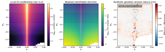
Figure 1: Historical analytic identifiability lens motivating the physical-shooting study. Left: local Jacobian condition number, which grows near k = 0 . Center: minimum singular value, showing the weakest identifiable direction. Right: change in identifiable- w_q error after adding the historical synthetic geodesic proxies; the mean MAE changes from 0.0225 to 0.0143. White regions are invalid or missing source-grid points and are not interpolated. The first two panels diagnose inverse-map geometry; the third records the original proxy experiment and must not be interpreted as physical ray tracing or geodesic shooting. Proxy augmentation does not resolve the exact k = 0 rank loss.
