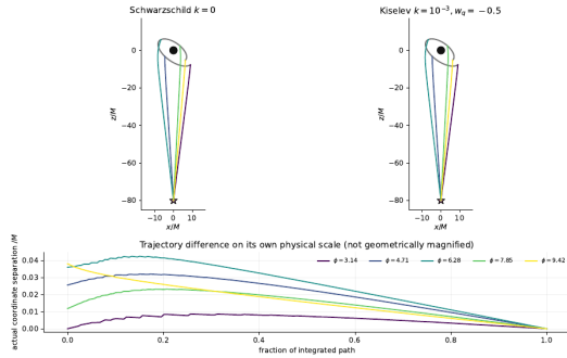
Figure 15: Matched-phase direct rays for Schwarzschild and k = 10^{-3} , w_q = -0.5 with M = 1 , r_p = 8M , r_o = 12M , and observer (0, 0, -80M) . The lower panel gives physical coordinate separation versus integrated path fraction. Differences are shown on their actual scale and are not geometrically magnified.
