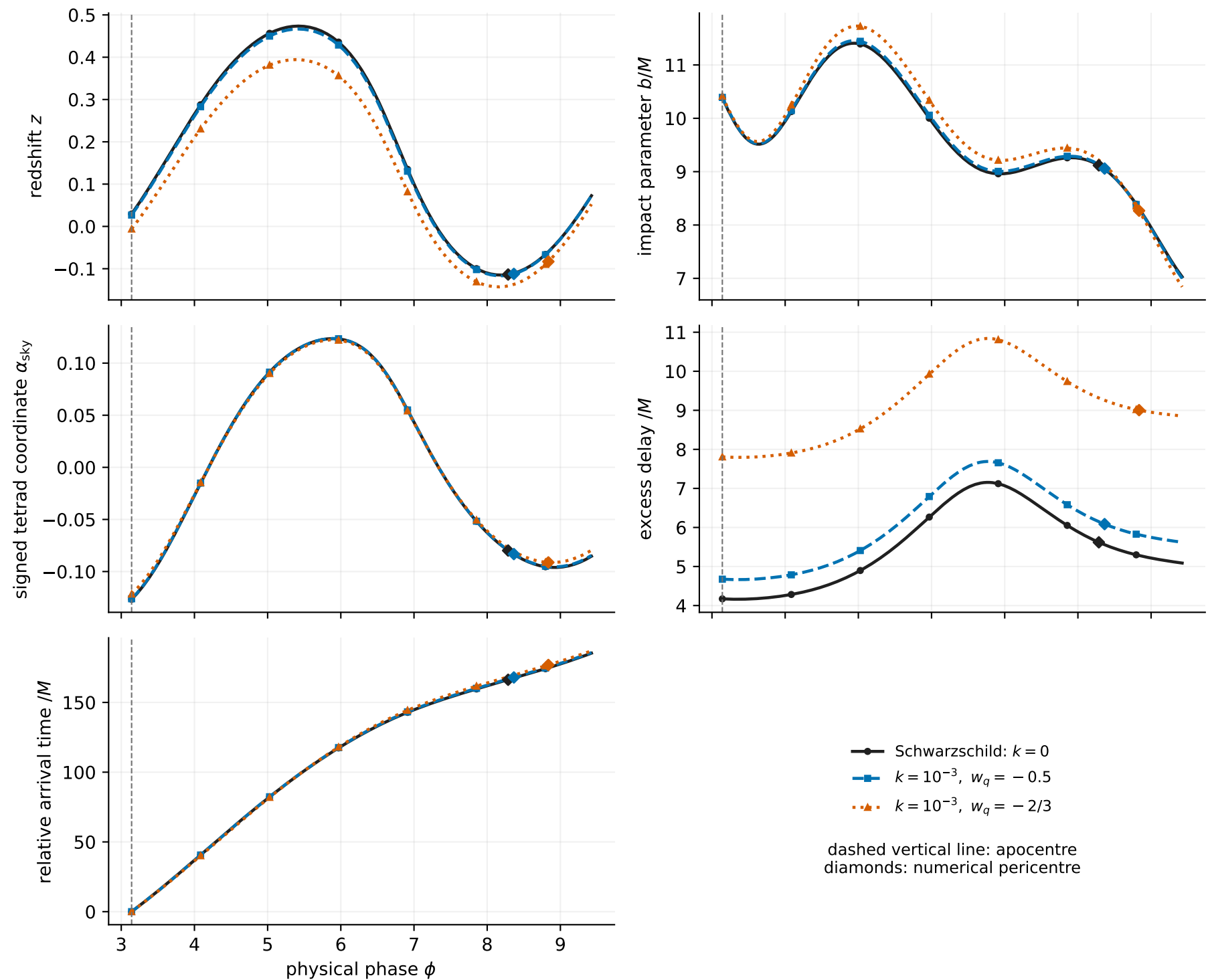
Physical shooting observables respond differently to the same spacetime parameters
