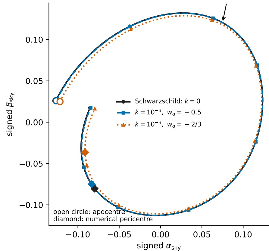
Observer-tetrad sky track increasing \phi
