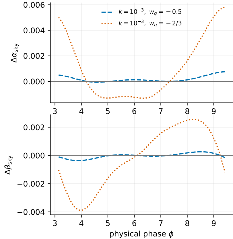
Matched-phase residuals from Schwarzschild
