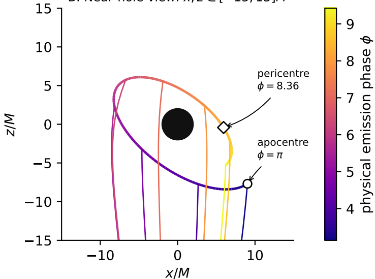
B. Near-hole view: x, z \in [-15, 15]M
