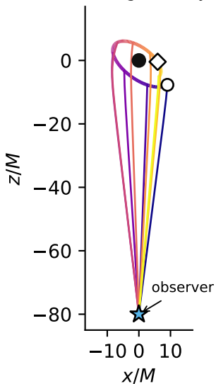
A. Full geometry
