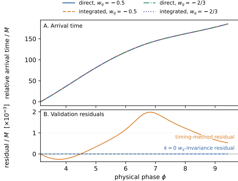
Figure 14: Schwarzschild arrival-time validation. The four phase-resolved series are the direct and redshift-integrated arrival-time constructions for each of two nominal w_q values. At k = 0 those values describe the same Schwarzschild geometry. In the lower panel, the orange residual checks timing consistency, T_{\text{direct}} - T_z , where T_z = \int (1+z) d\tau_{\text{emit}} , and the blue residual checks exact k = 0 w_q invariance, T_{\text{direct}}(w_q = -0.5) - T_{\text{direct}}(w_q = -2/3) . Both are shown on their actual numerical scales. The independently integrated T_z is a validation quantity, not the timing feature used for ML inference.
