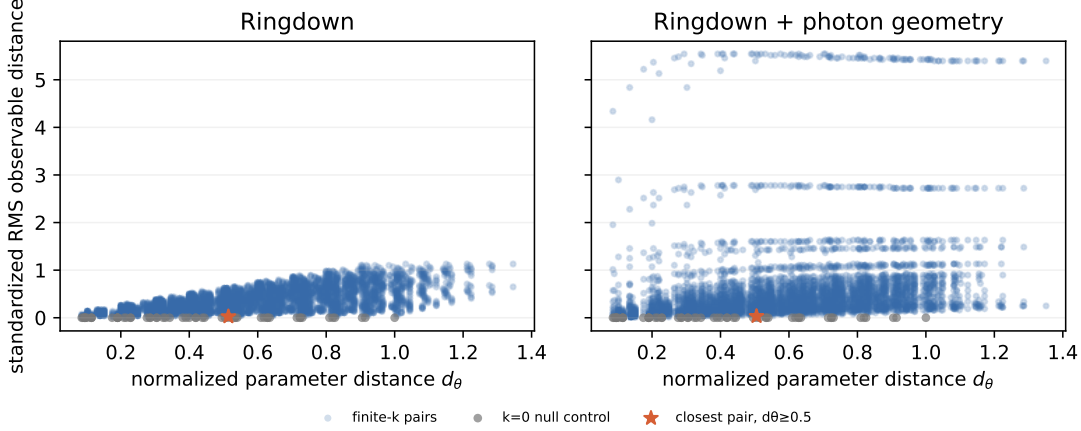
Figure 17: All-pairs finite-domain ambiguity audit. The horizontal axis is normalized parameter distance and the vertical axis is RMS standardized observable distance. Grey k = 0 pairs show the required structural degeneracy; distant finite- k pairs are the relevant sampled-domain diagnostic. Stars mark the closest finite- k pair with d_\theta \geq 0.5 . This plot tests only the sampled physical grid and does not establish continuous global injectivity.
