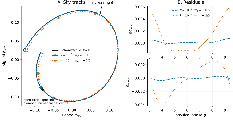
Figure 15: Static-observer-tetrad sky tracks and actual-scale residuals for the same M = 1 , r_p = 8M , r_a = 12M , observer (0, 0, -80M) direct-branch benchmark. Open circles mark \phi = \pi apocentre, diamonds mark numerical pericentre, and the arrow gives increasing phase. Residuals are pointwise differences from Schwarzschild at exactly matched successful phases; they are neither normalized for visibility nor interpolated across failures.
