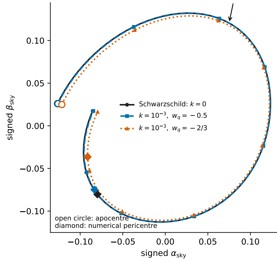
A. Sky tracks increasing \phi
