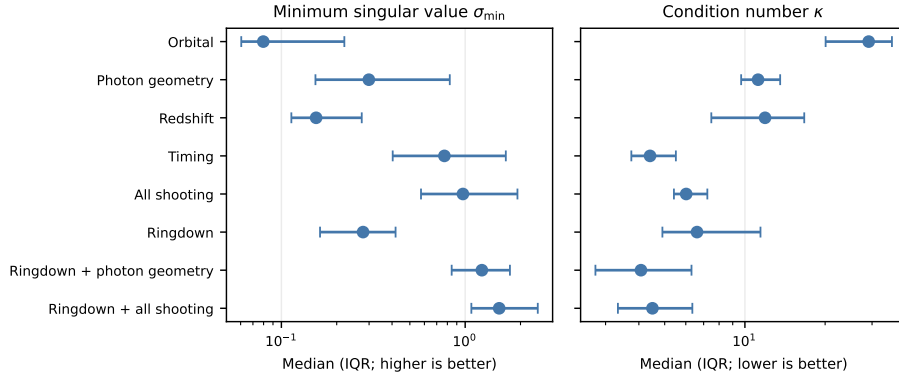
Figure 7: Nominal 81-phase grid-wide median and interquartile summaries of \sigma_{\min} and condition number. Photon geometry provides the clearest complement to ringdown; the separate 161-phase audit is reported in the text.
