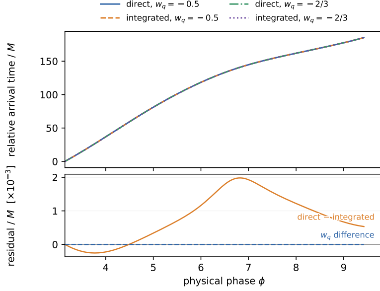
Figure 15: Schwarzschild arrival-time validation. Four arrival-time phase-resolved series are plotted. The two nominal w_q cases coincide because the k = 0 geometry is Schwarzschild, while the direct and integrated-redshift constructions agree within numerical quadrature error. The lower panel shows direct minus integrated arrival time for w_q = -0.5 and the direct-arrival difference between w_q = -0.5 and w_q = -2/3 on their actual numerical scales.
