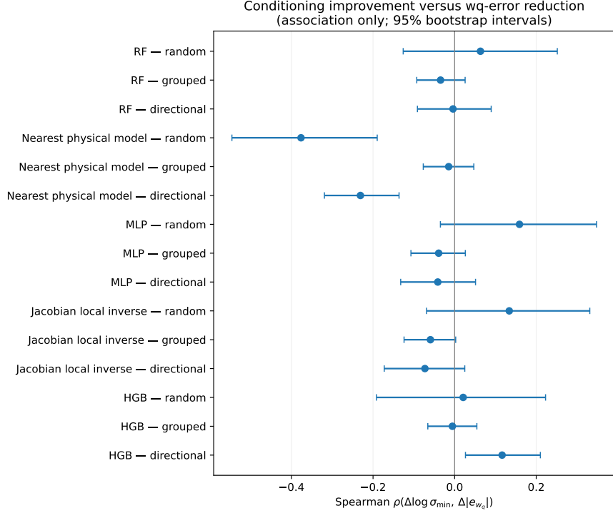
Figure 14: Spearman association between the change in log minimum singular value and the reduction in absolute identifiable- w_q error when photon geometry is added to ringdown. Points show method/protocol estimates and bars are 95% bootstrap intervals. Associations are descriptive and do not imply causation.
