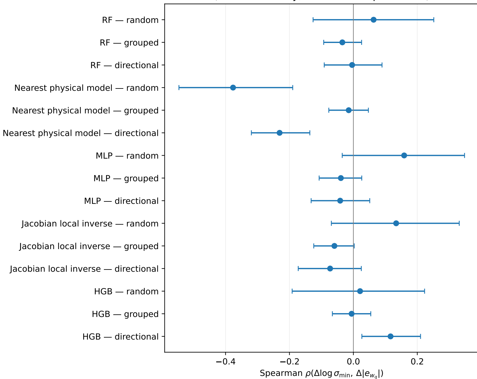
Conditioning improvement versus wq-error reduction (association only; 95% bootstrap intervals)
