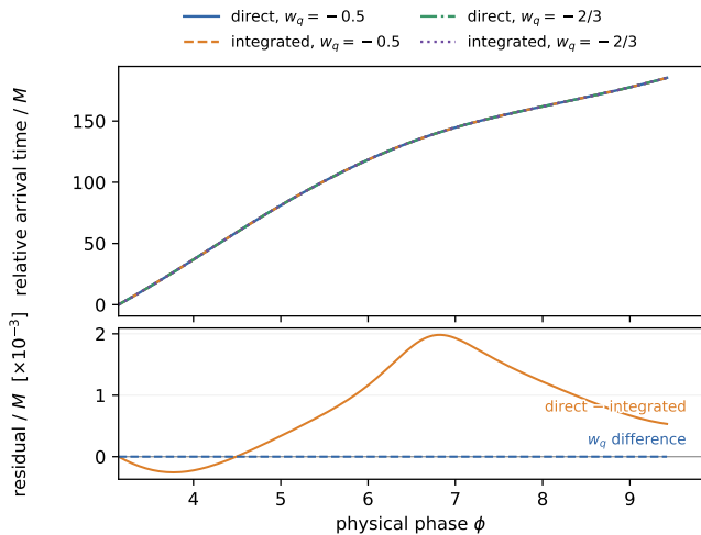
Figure 14: Schwarzschild arrival-time validation. Four arrival-time curves are plotted. The two nominal w_q cases coincide because the k = 0 geometry is Schwarzschild, while the direct and integrated-redshift constructions agree within numerical quadrature error. The lower panel shows direct minus integrated arrival time for w_q = -0.5 and the direct-arrival difference between w_q = -0.5 and w_q = -2/3 on their actual numerical scales.
