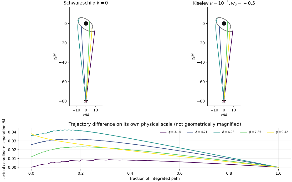
Figure 15: Matched-phase direct rays for Schwarzschild and k = 10^{-3} , w_q = -0.5 with M = 1 , r_p = 8M , r_a = 12M , and observer (0,0,-80M) . The lower panel gives physical coordinate separation versus integrated path fraction. Differences are shown on their actual scale and are not geometrically magnified.
