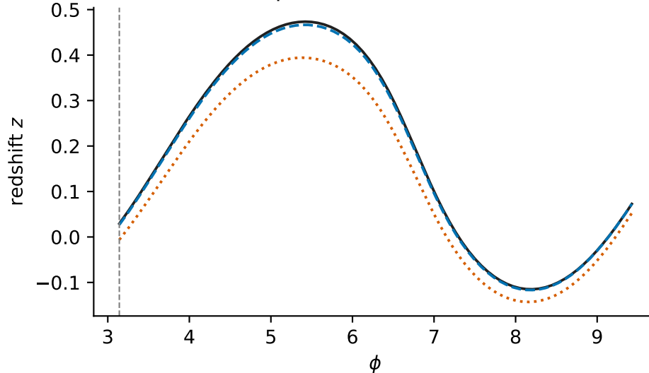
phase observable
