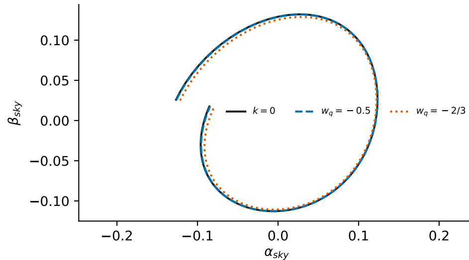
observer sky
