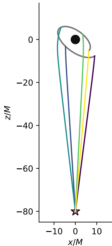
Schwarzschild k = 0
