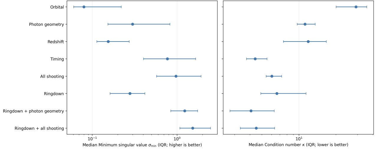
Figure 7: Grid-wide median and interquartile summaries of \sigma_{\min} and condition number. Photon geometry provides the clearest complement to ringdown.
