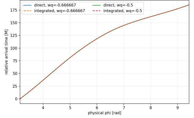
Figure 1: Schwarzschild shooting validation. Physical phase begins at \phi = \pi at apocentre. Direct arrival time and the integrated-redshift curve share only the first-phase additive constant.
